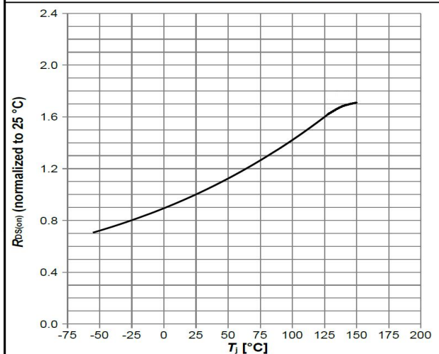
Diagram 9: Normalized drain-source on resistance
