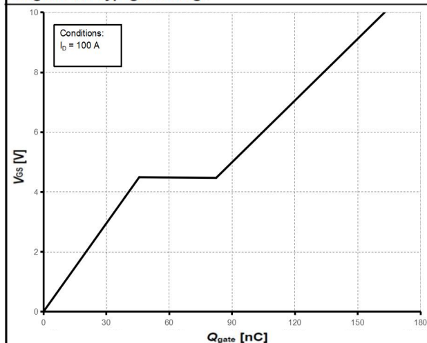
Diagram 11: Typ. gate charge
