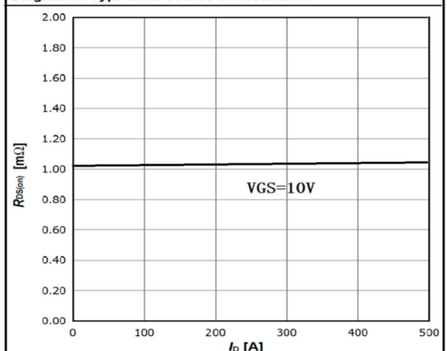
Diagram 6: Typ. drain-source on resistance
