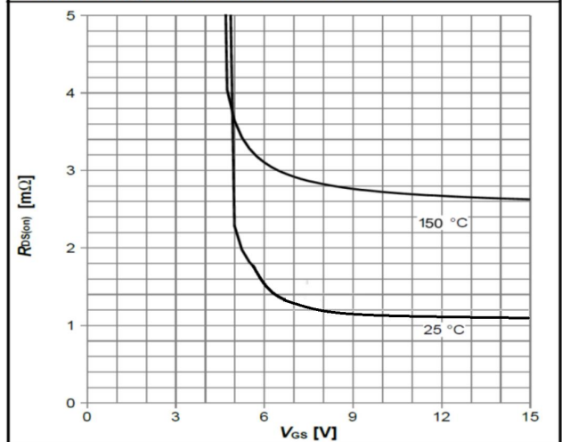
Diagram 8: Typ. drain-source on resistance
