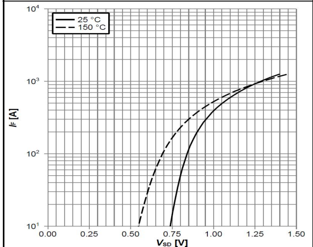
Diagram 10: Typ. forward characteristics of reverse diode
