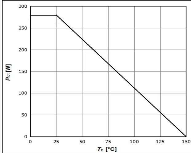
Diagram 1: Power dissipation
