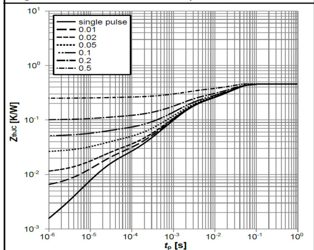
Diagram 4: Max. transient thermal impedance
