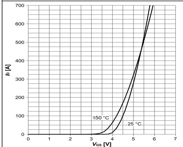
Diagram 7: Typ. transfer characteristics
