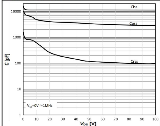
Diagram 12: Typ. capacitances
