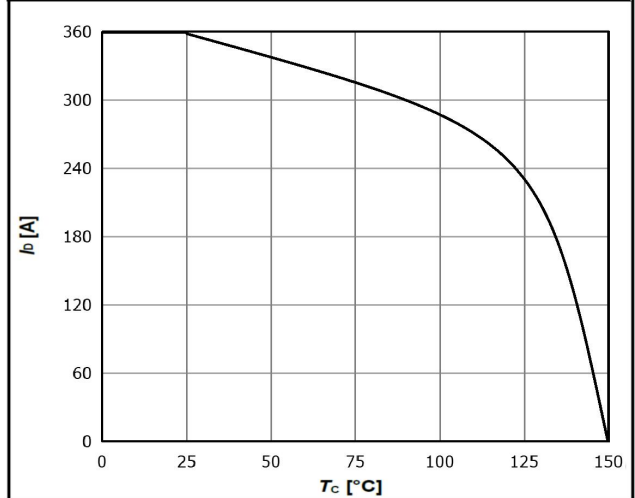
Diagram 2: Drain current
