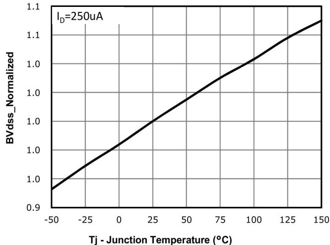
Fig 8: BV_{dss} vs. Temperature
