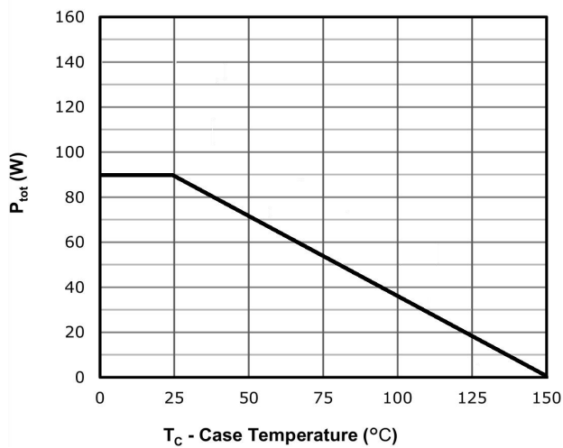
Fig 9: Power Dissipation
