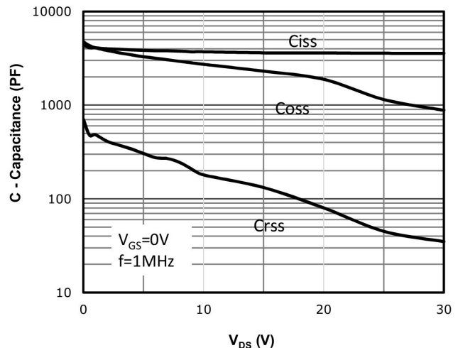
Fig 6: Capacitance Characteristics
