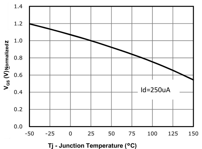
Fig 12: Vgs(th) vs. Temperature
