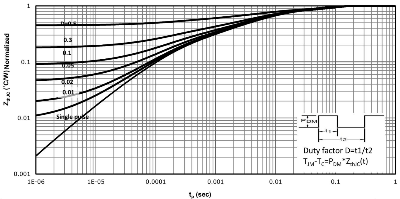
Fig 14: Max. Transient Thermal Impedance
