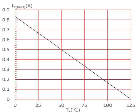
FIG.5: On-state characteristics
