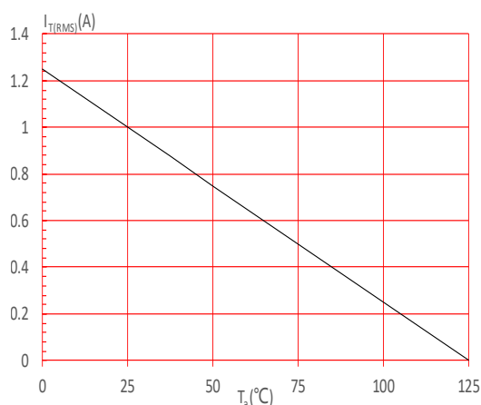
FIG.5: On-state characteristics
