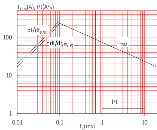
FIG.5: Non-repetitive surge peak on-state current for a sinusoidal pulse with width t_p < 20ms , and corresponding value of I^2t ( I - II : dl/dt < 30A/\mu s ; III - IV : dl/dt < 20A/\mu s )
