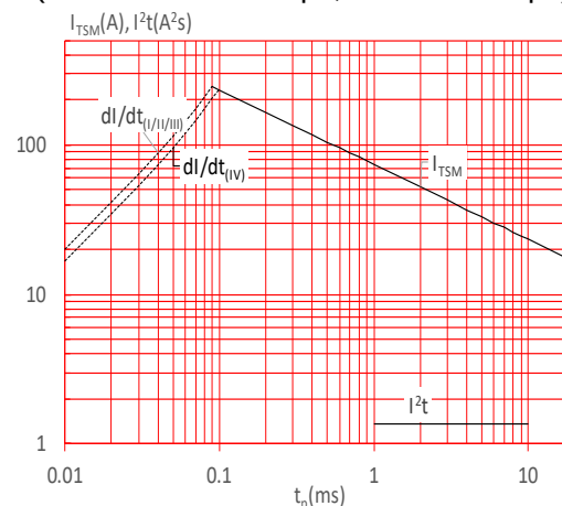
FIG.6: Non-repetitive surge peak on-state current for a sinusoidal pulse with width t_p < 20ms , and corresponding value of I^2t (I - II - III: di/dt < 50A/μs ; IV: di/dt < 30A/μs )
