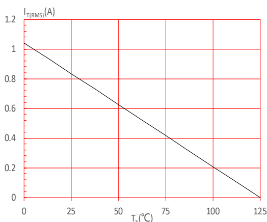
FIG.5: On-state characteristics
