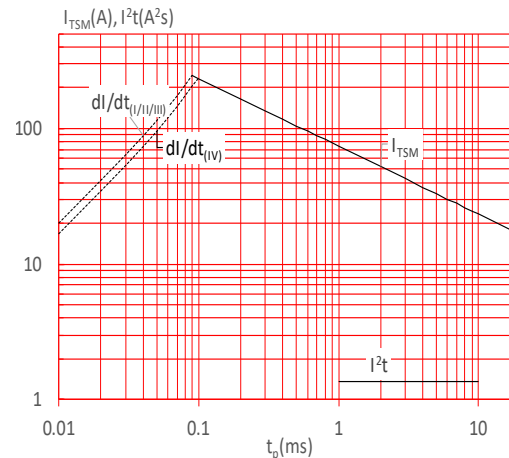
FIG.6: Non-repetitive surge peak on-state current for a sinusoidal pulse with width t_p < 20ms , and corresponding value of I^2t (I - II - III: di/dt < 50A/\mu s ; IV: di/dt < 30A/\mu s )
