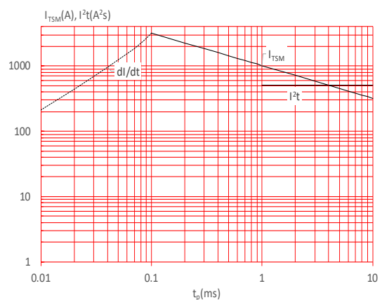
FIG.6: Non-repetitive surge peak on-state current for a sinusoidal pulse with width t_p < 10ms , and corresponding value of I^2t ( di/dt < 200A/μs )
