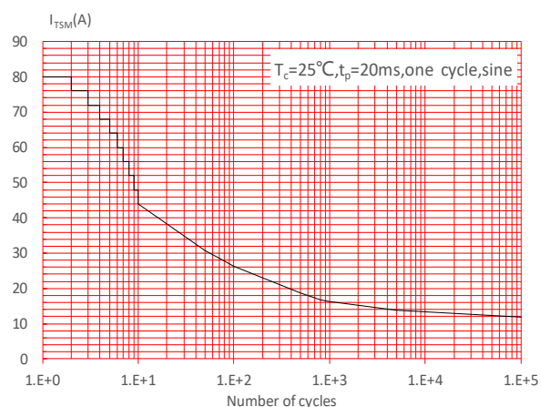
FIG.6: Non-repetitive surge peak on-state current for a sinusoidal pulse with width t_p < 20ms , and corresponding value of I^2t ( dI/dt < 100A/μs )
