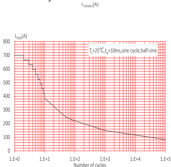
FIG.5: Non-repetitive surge peak on-state current for a sinusoidal pulse with width t_p < 10\text{ms} , and corresponding value of I^2t ( di/dt < 200\text{A}/\mu\text{s} )
