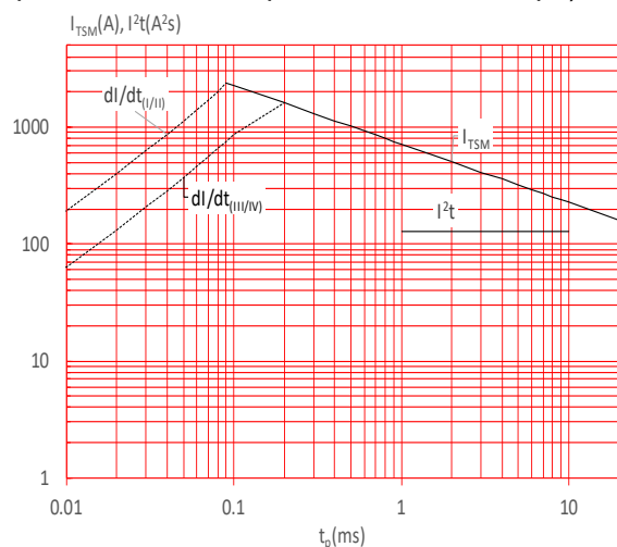
FIG.5: Non-repetitive surge peak on-state current for a sinusoidal pulse with width t_p < 20ms , and corresponding value of I^2t ( I - II : di/dt < 100A/\mu s ; III-IV : di/dt < 50A/\mu s )
