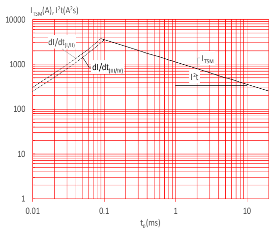
FIG.5: Non-repetitive surge peak on-state current for a sinusoidal pulse with width t_p < 20\text{ms} , and corresponding value of I^2t (I - II: di/dt < 100\text{A}/\mu\text{s} ; III-IV: di/dt < 50\text{A}/\mu\text{s} )
