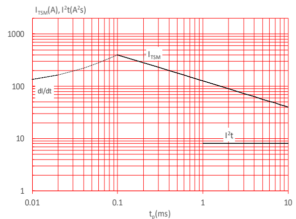
FIG.6: Non-repetitive surge peak on-state current for a sinusoidal pulse with width t_p < 10ms , and corresponding value of I^2t ( di/dt < 50A/μs )
