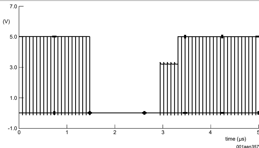
Figure 27. Example 2: overshoot_t1 = 0d; overshoot_t2 = 5d
