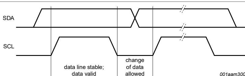
Figure 17. Bit transfer on the I 2 C-bus
