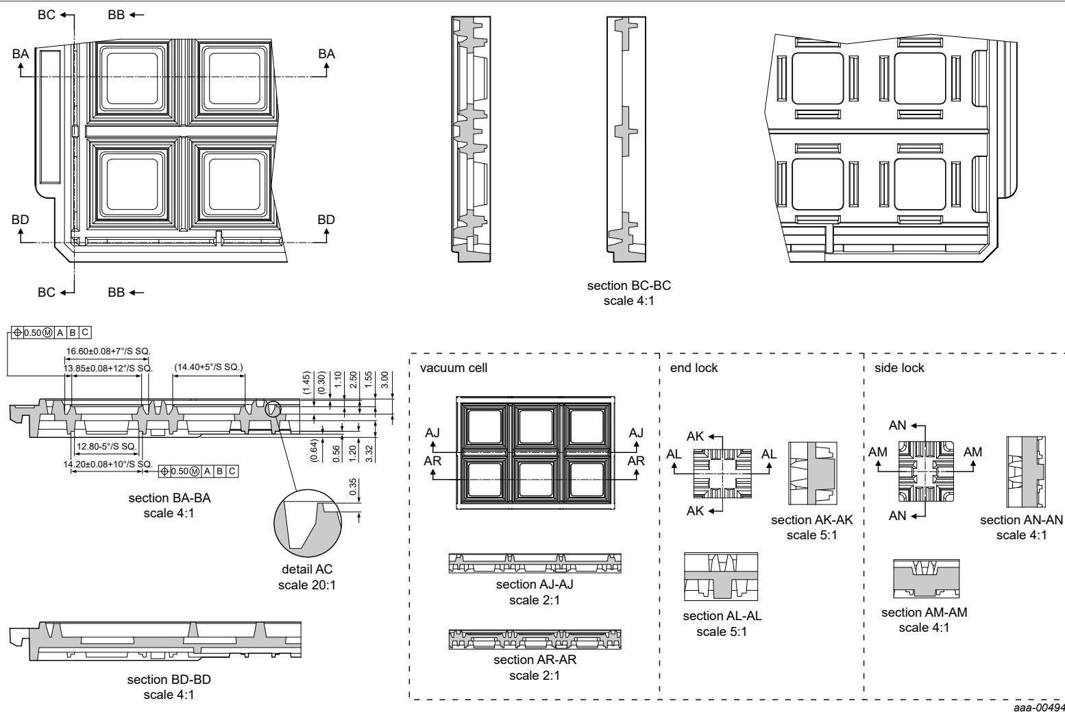
Figure 47. Tray details
