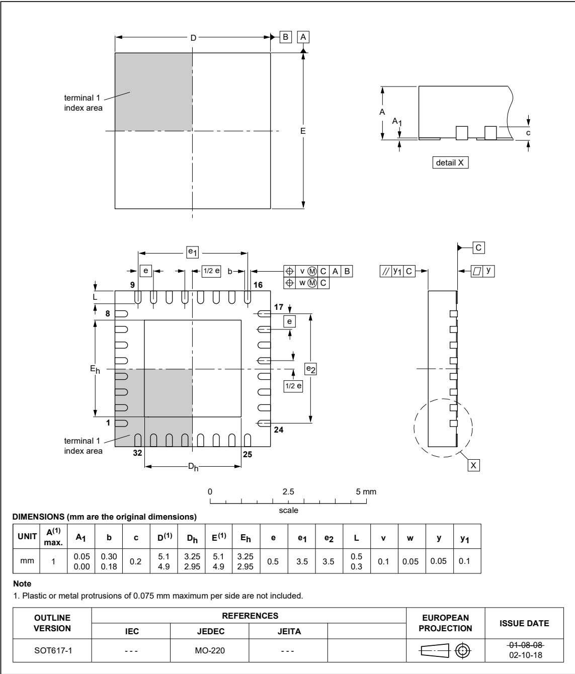
Figure 37. Package outline SOT-617-1 (HVQFN32)
