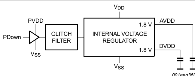
Figure 33. Internal PDown to voltage regulator logic
