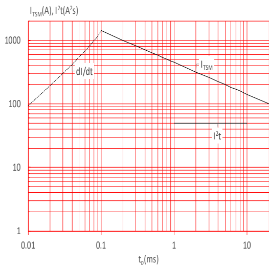
FIG.5: Non-repetitive surge peak on-state current for a sinusoidal pulse with width t_p < 20ms , and corresponding value of I^2t ( di/dt < 100A/\mu s )
