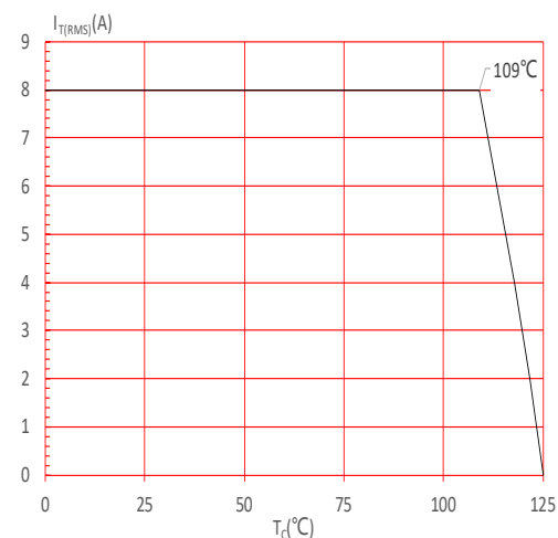
FIG.4: On-state characteristics
