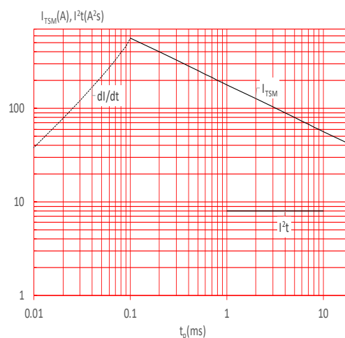
FIG.6: Non-repetitive surge peak on-state current for a sinusoidal pulse with width t_p < 20ms , and corresponding value of I^2t ( di/dt < 50A/\mu s )
