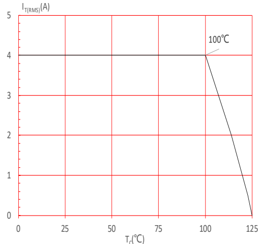
FIG.2: RMS on-state current versus case temperature
