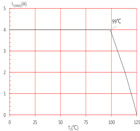
FIG.2: RMS on-state current versus case temperature
