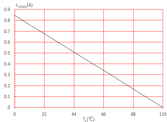
FIG.5: On-state characteristics
