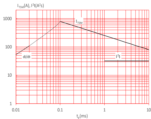
FIG.6: Non-repetitive surge peak on-state current for a sinusoidal pulse with width t_p < 10ms , and corresponding value of I^2t ( di/dt < 100A/μs )
