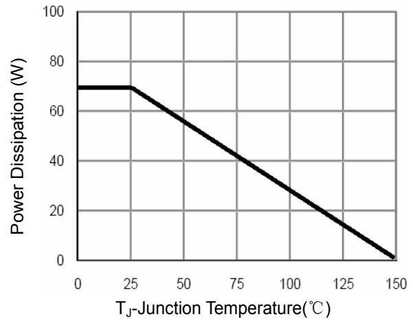
Figure 9 Power De-rating
