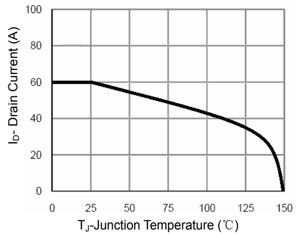
Figure 10 Current De-rating
