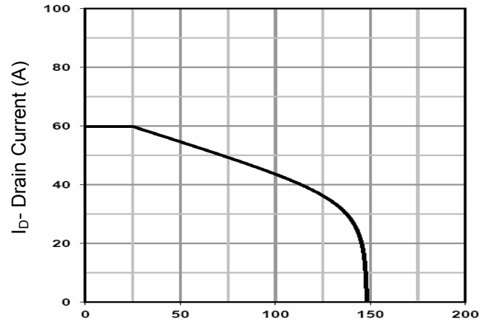
Figure 9 Current De-rating
