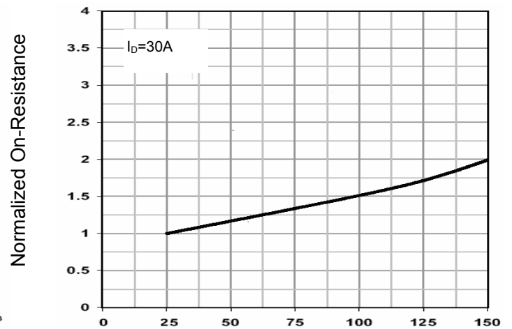
Figure 10 R_{DS(on)} -Junction Temperature
