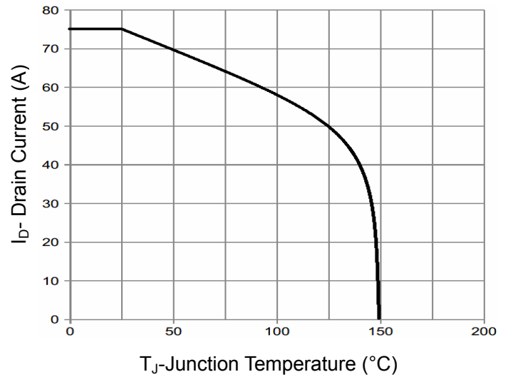
Figure 9 Current De-rating
