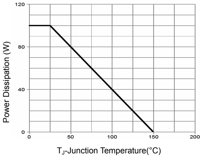
Figure 7 Power De-rating
