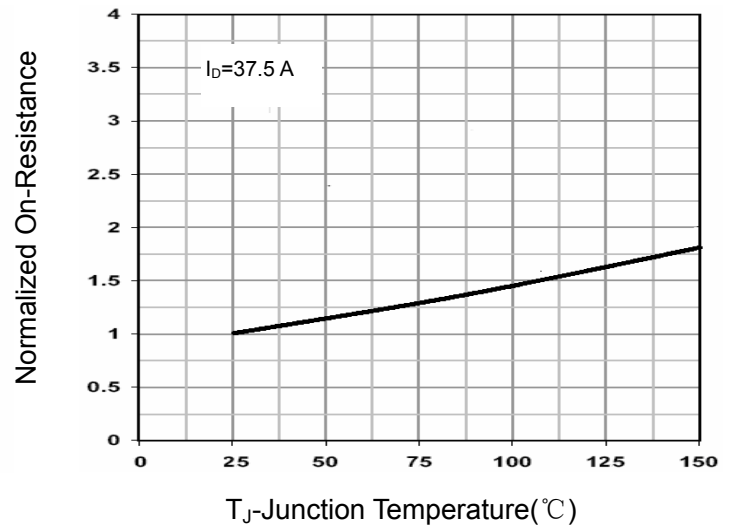
Figure 10 Rdson-Junction Temperature
