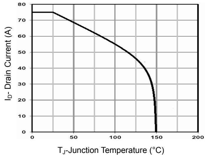
Figure 9 Current De-rating
