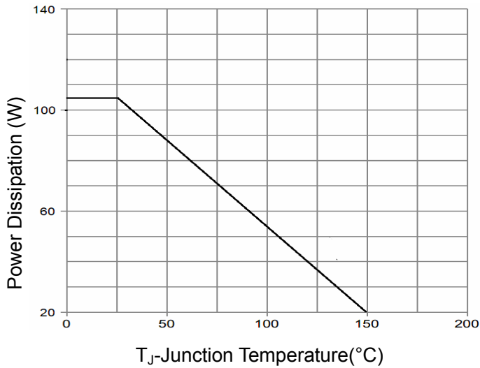
Figure 7 Power De-rating
