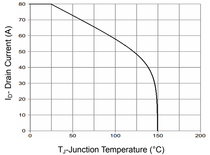
Figure 9 Current De-rating
