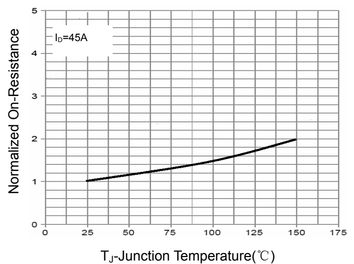
Figure 10 R_{DS(on)} -Junction Temperature
