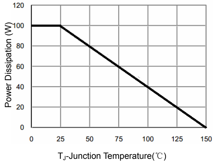
Figure 9 Power De-rating
