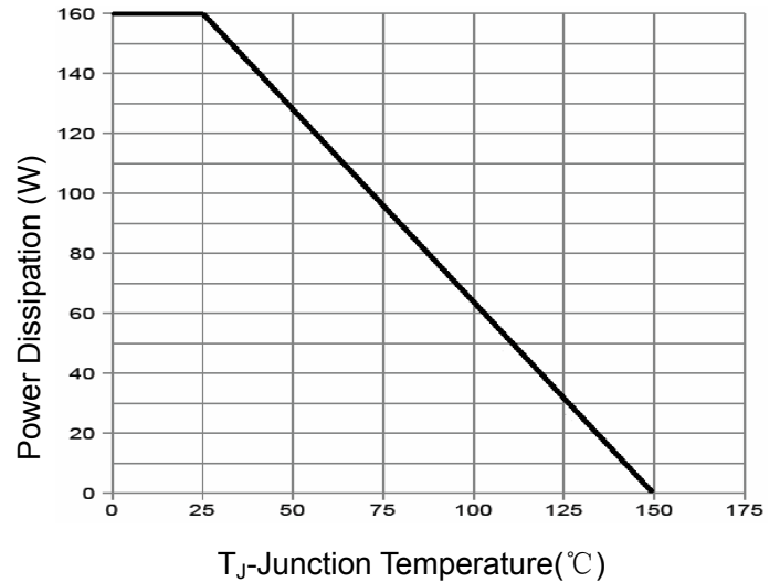
Figure 9 Power De-rating
