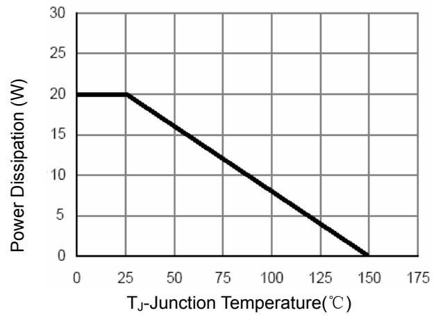
Figure 9 Power De-rating
