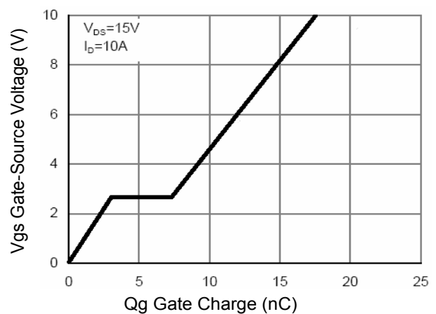
Figure 5 Gate Charge
