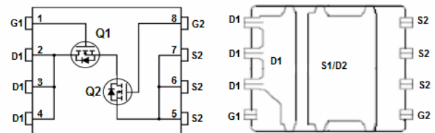
pin assignment
