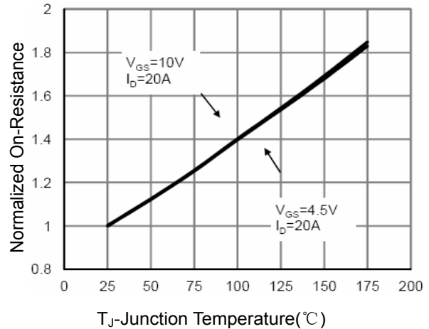
Figure 4 Rdson-Junction Temperature
