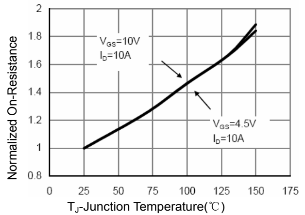
Figure 4 Rdson-Junction Temperature
