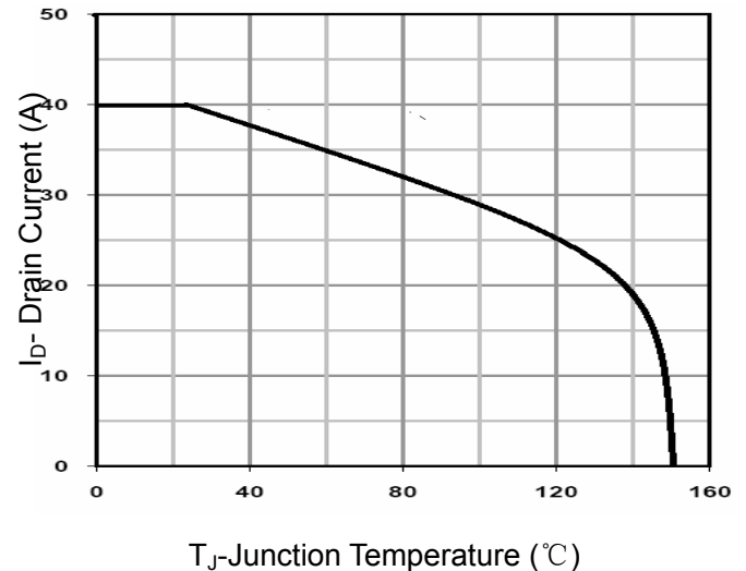
Figure 10 Current De-rating
