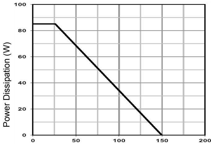
Figure 7 Power De-rating
