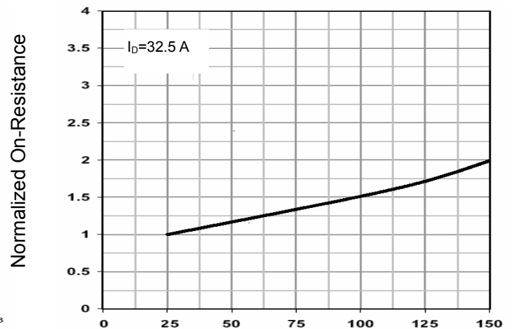
Figure 10 Rdson-Junction Temperature
