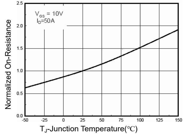
Figure 4 Rdson-Junction Temperature
