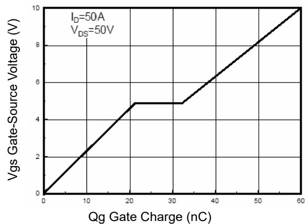
Figure 5 Gate Charge
