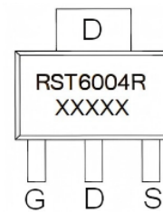
SOT-223-3L view
