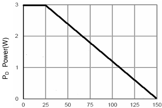
Figure 3 Power Dissipation
