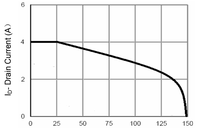
Figure 4 Drain Current
