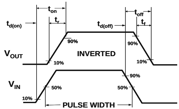
Figure 2 Switching Waveforms
