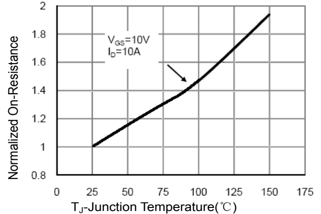
Figure 4 Rdson-Junction Temperature
