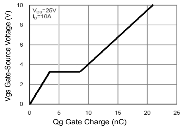
Figure 5 Gate Charge
