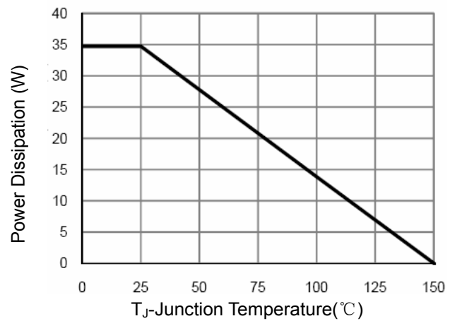
Figure 9 Power De-rating
