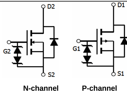
Schematic diagram
