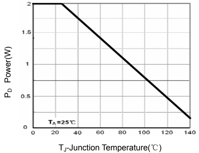
Figure 9 Power Dissipation
