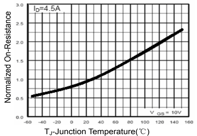
Figure 4 Rdson-Junction Temperature
