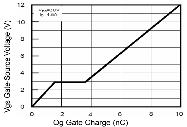
Figure 5 Gate Charge
