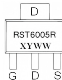
SOT-223-3L view
