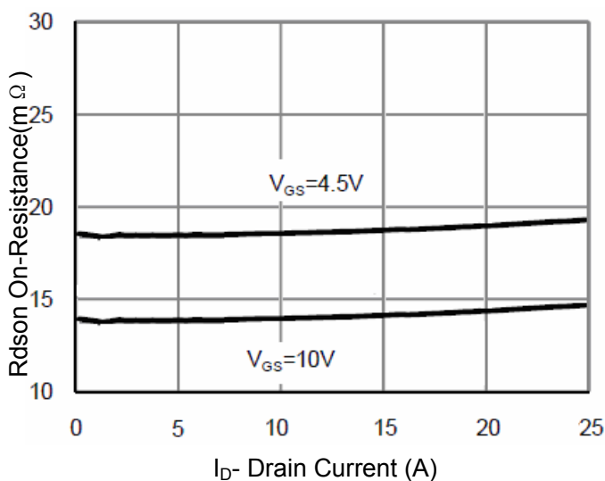
Figure 5 Drain-Source On-Resistance
