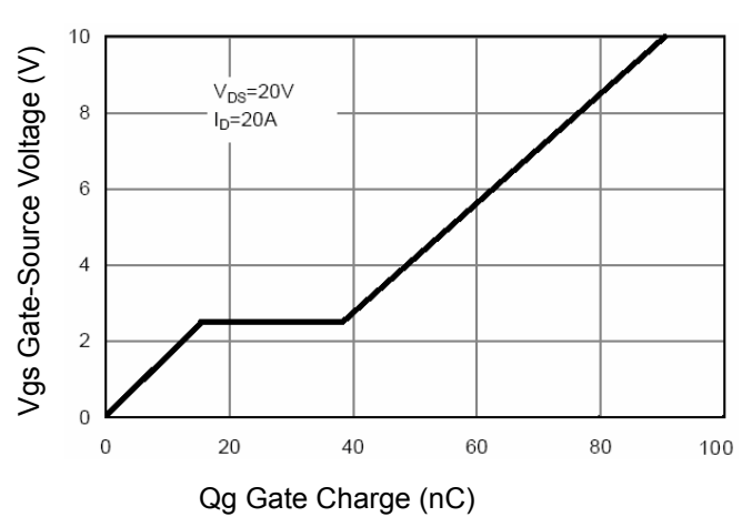
Figure 5 Gate Charge
