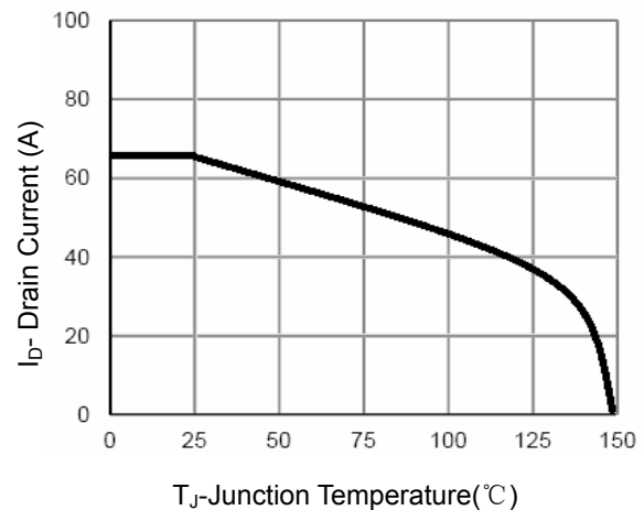
Figure 10 Current De-rating
