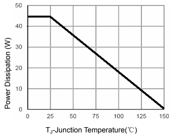
Figure 9 Power De-rating
