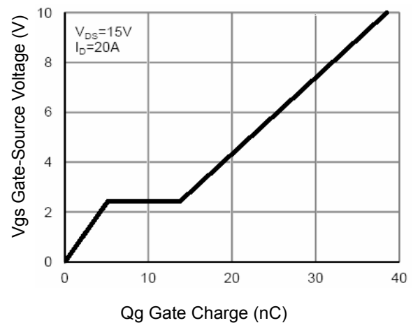
Figure 5 Gate Charge
