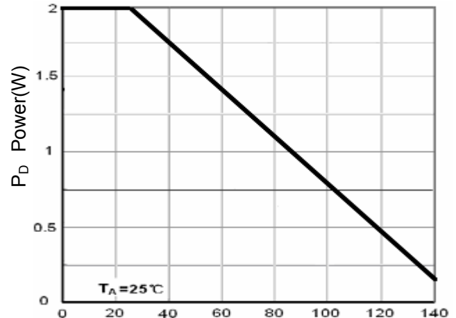
Figure 8 Power Dissipation
