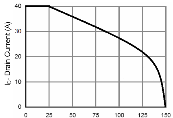
TJ-Junction Temperature(°C) Figure10 ID Current- Junction Temperature
