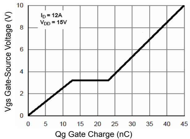
Figure 5 Gate Charge
