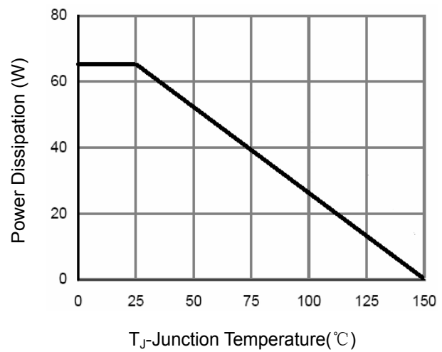
Figure 9 Power De-rating
