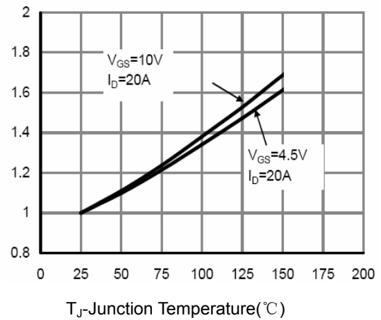
Figure 4 Rdson-Junction Temperature
