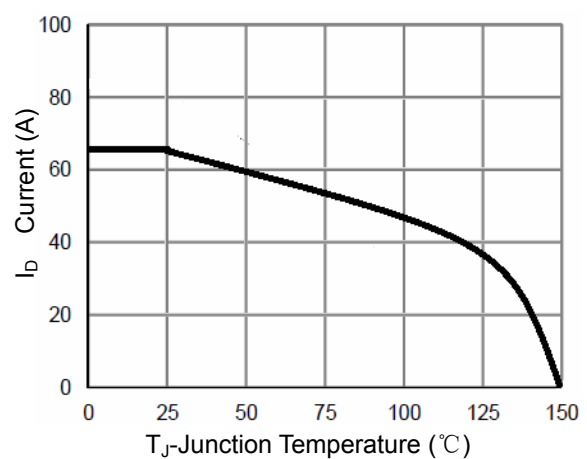
Figure 10 Current- Junction Temperature
