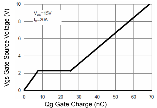
Figure 5 Gate Charge
