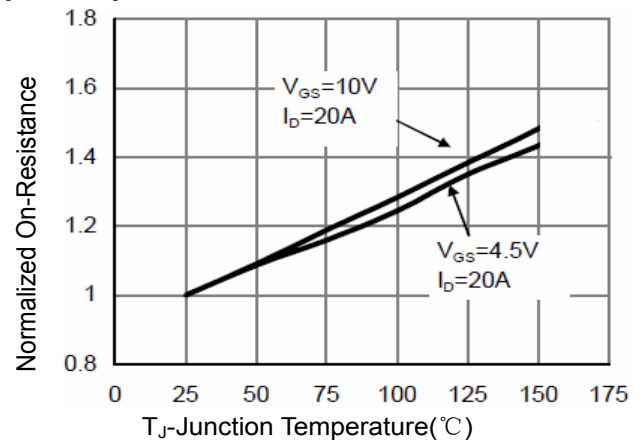
Figure 4 Rdson-Junction Temperature
