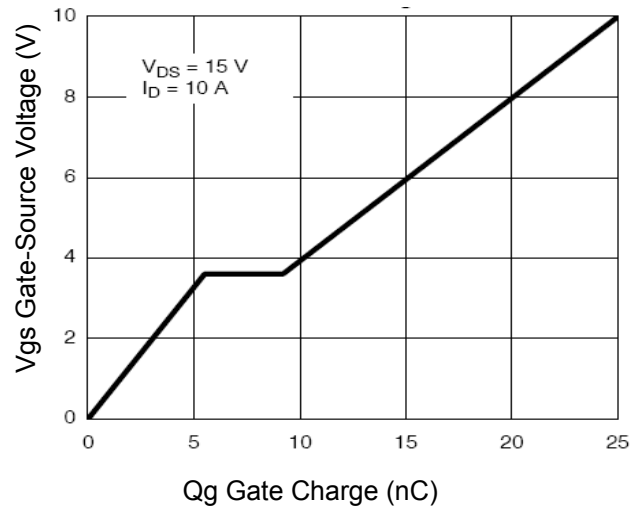
Figure 5 Gate Charge
