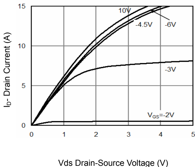
Figure 5 Output Characteristics
