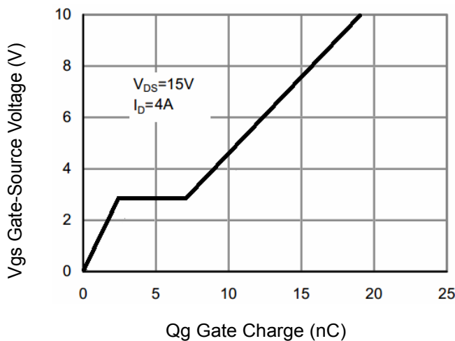
Figure 11 Gate Charge
