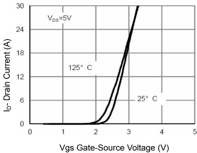
Figure 7 Transfer Characteristics
