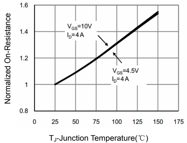
Figure 8 Drain-Source On-Resistance
