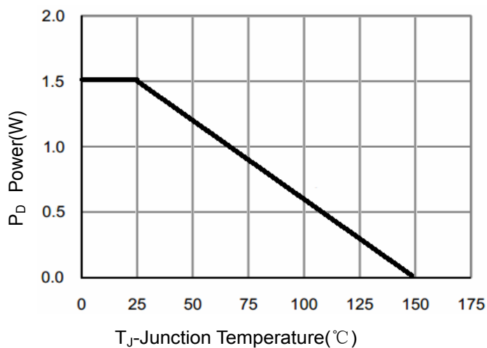
Figure 3 Power Dissipation
