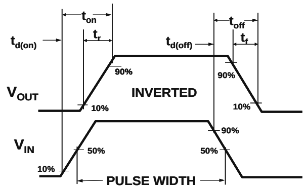
Figure 2 Switching Waveforms
