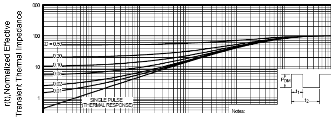
Vds Drain-Source Voltage (V) Figure 13 Safe Operation Area
